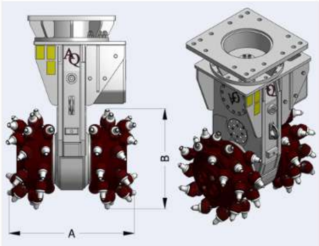
Quantity of cutter bits for standard drums: 56
