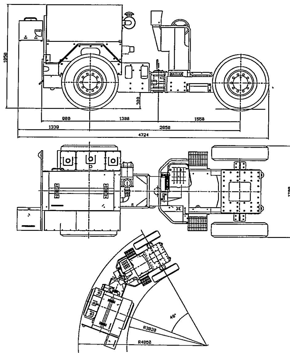
Fig. 1. Dimensioned drawing
