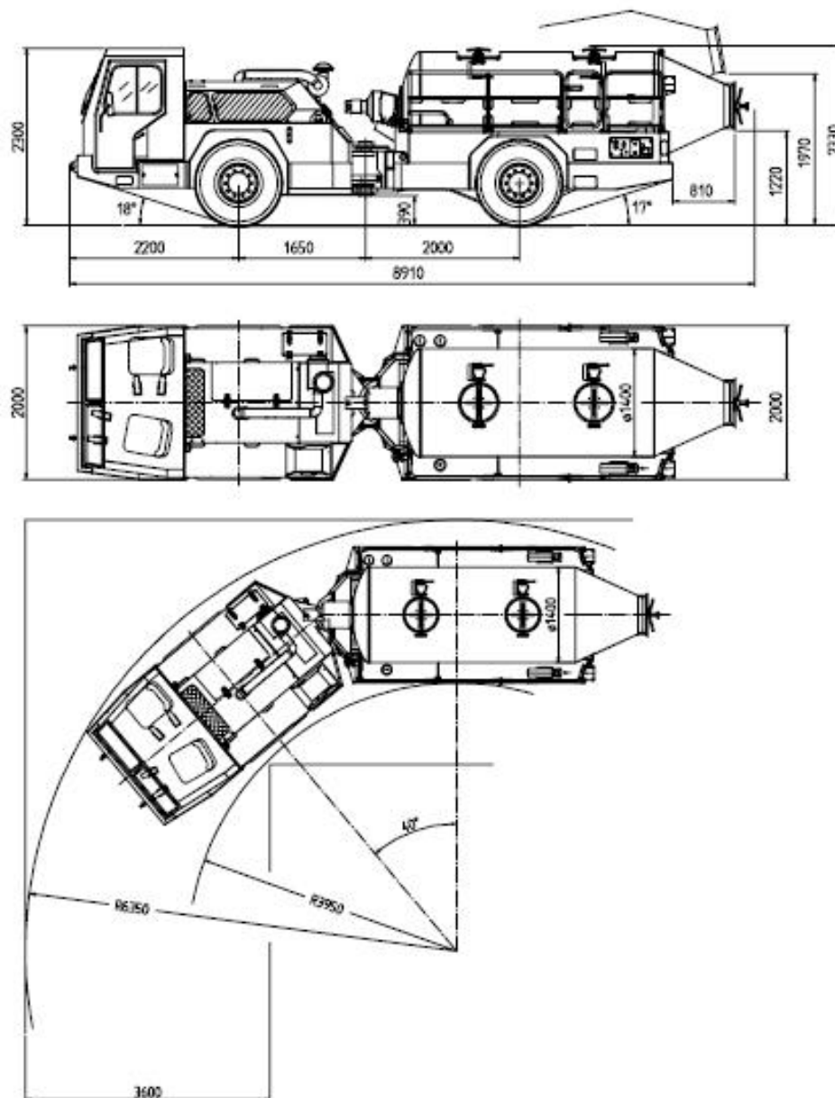
Fig. 1. Dimensioned drawing
